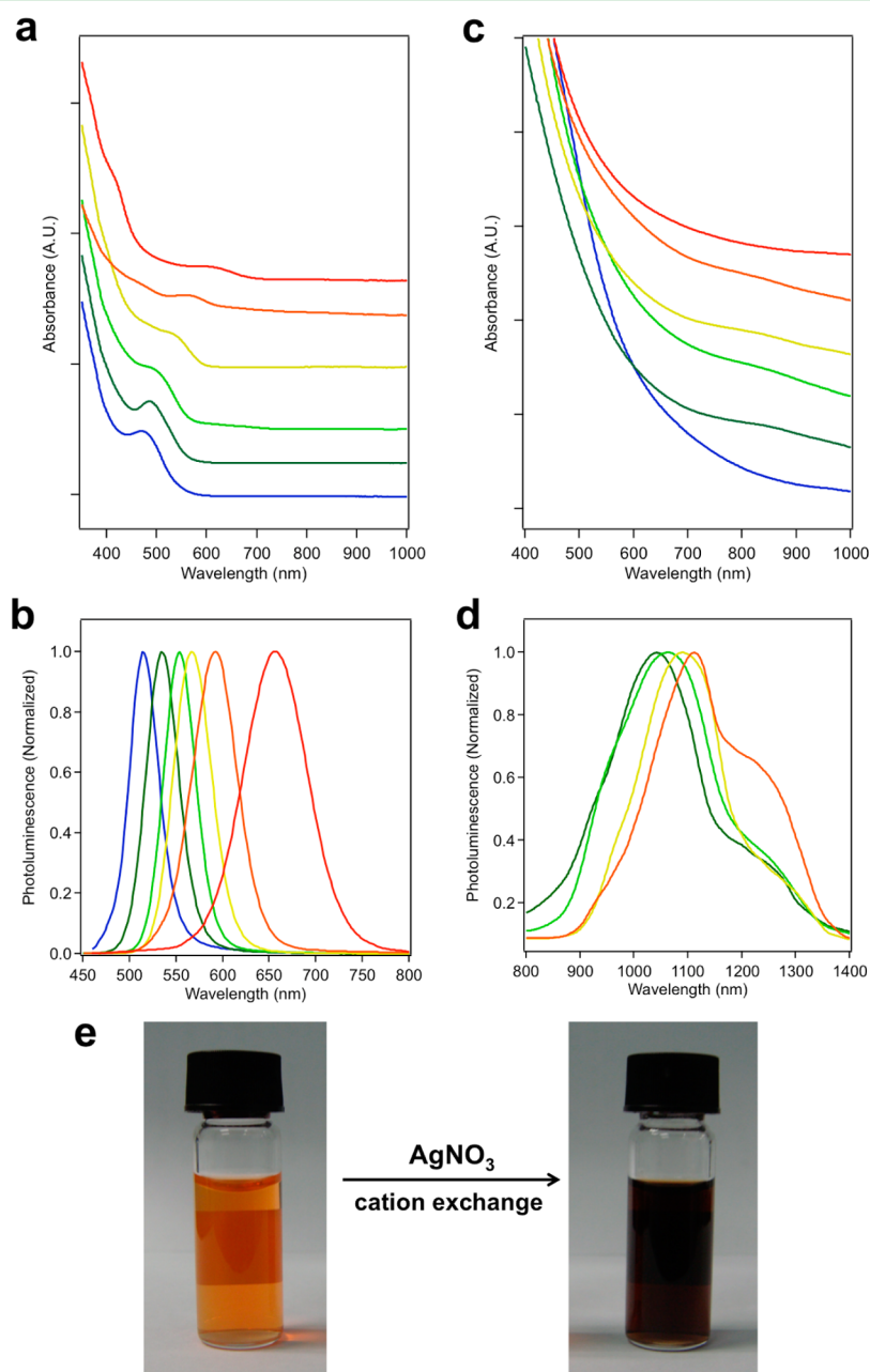
Figure 1. Optical characterization of CdTe QDs and Ag 2 Te QDs. (a) Absorption spectra of CdTe QDs synthesized with various reaction time (from bottom to top: 15, 30, 45, 60, 90, and 150 min). (b) Photoluminescence spectra of CdTe QDs synthesized with various reaction time (from left to right: 15, 30, 45, 60, 90, and 150 min). (c) Absorption spectra of Ag 2 Te QDs prepared from CdTe QDs via cation exchange (The corresponding CdTe QDs and Ag 2 Te QDs are depicted in the same color). (d) Photoluminescence spectra of Ag 2 Te QDs prepared from CdTe QDs via cation exchange (The corresponding CdTe QDs and Ag 2 Te QDs are depicted in the same color). The cation exchange products prepared from the smallest and biggest CdTe QDs are not luminescent and not shown in the figure. (e) Photographs of the CdTe QDs (left) and the Ag 2 Te QDs (right) prepared via cation exchange. (A rectangular label attached to the back of the bottle can be visualized through the CdTe QDs solution (left)).
